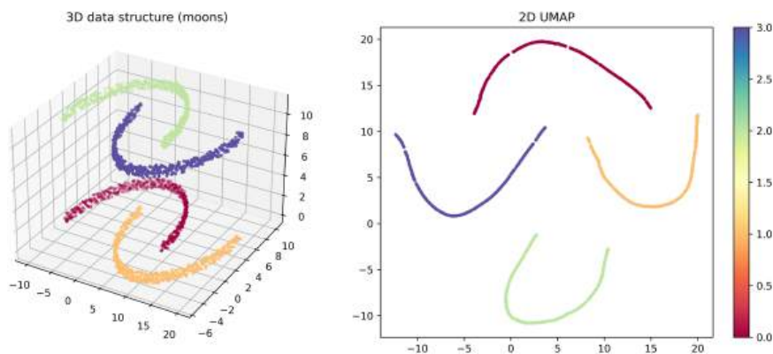
Figure 18.2 Projection of three-dimensional shapes (moons) onto a two-dimensional plane using UMAP.
