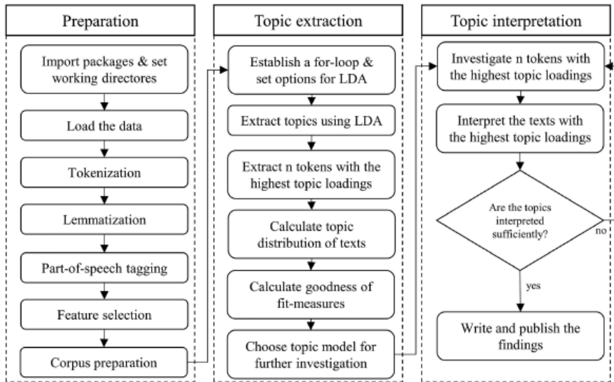
Figure 17.1 LDA workflow.
