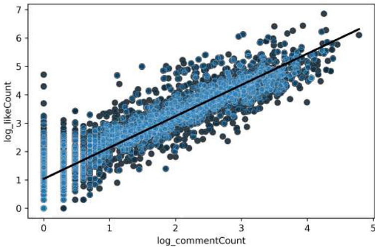
Figure 14.7 Scatterplot and regression plot highlighting the association between the logarithmized number of comments and logarithmized number of likes per YouTube video under observation.
