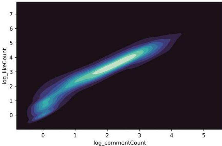
Figure 14.8 Two-dimensional KDE plot illustrating the association between logarithmized comments and likes.
