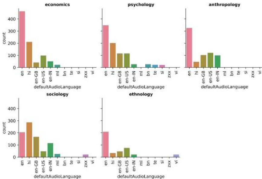
Figure 14.6 Bar plot displaying the number of YouTube videos per language and academic discipline.
