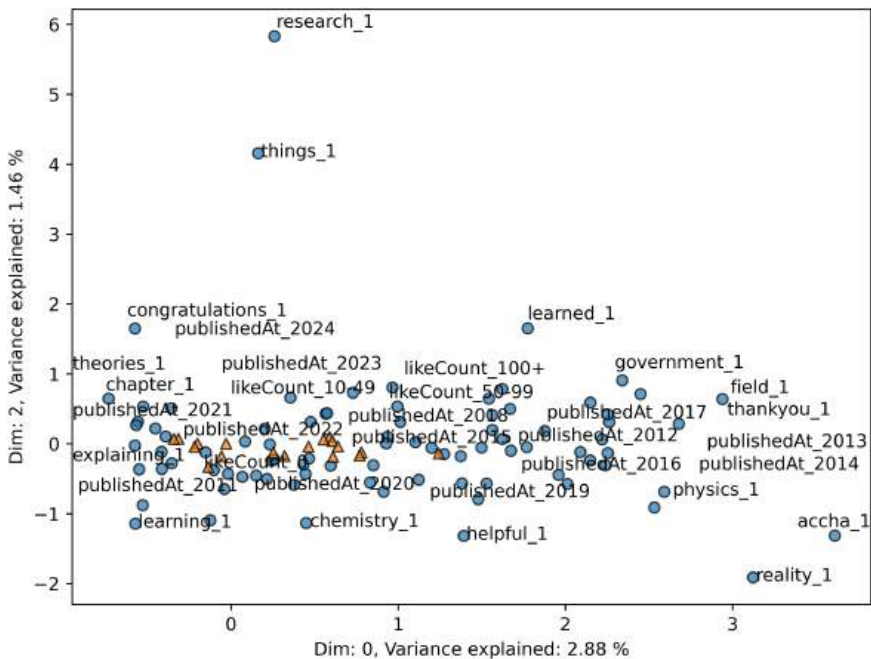
Figure 15.6 Biplot of the position of the active and passive variables on dimensions 0 and 2.
