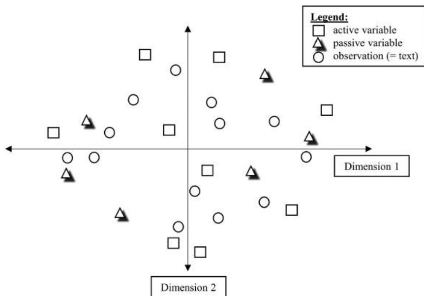
Figure 15.1 Exemplary depiction of a space extracted by GDA, called biplot, including active variables, passive variables, and observations.
