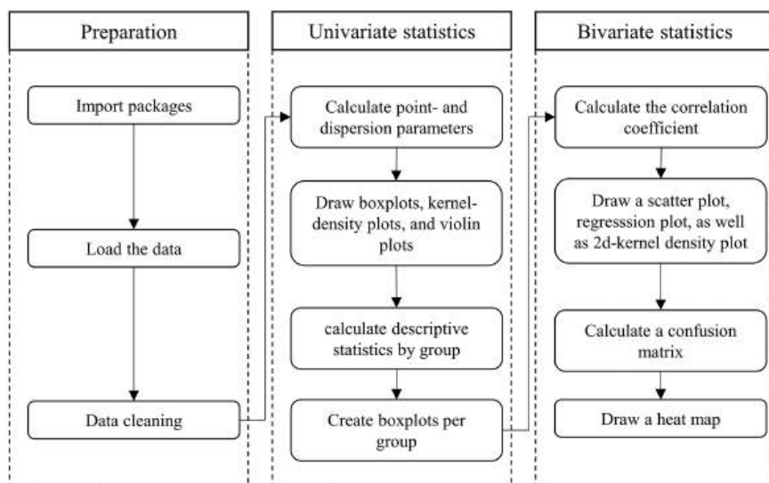
Figure 14.1 Workflow of the descriptive analysis of video metadata.
