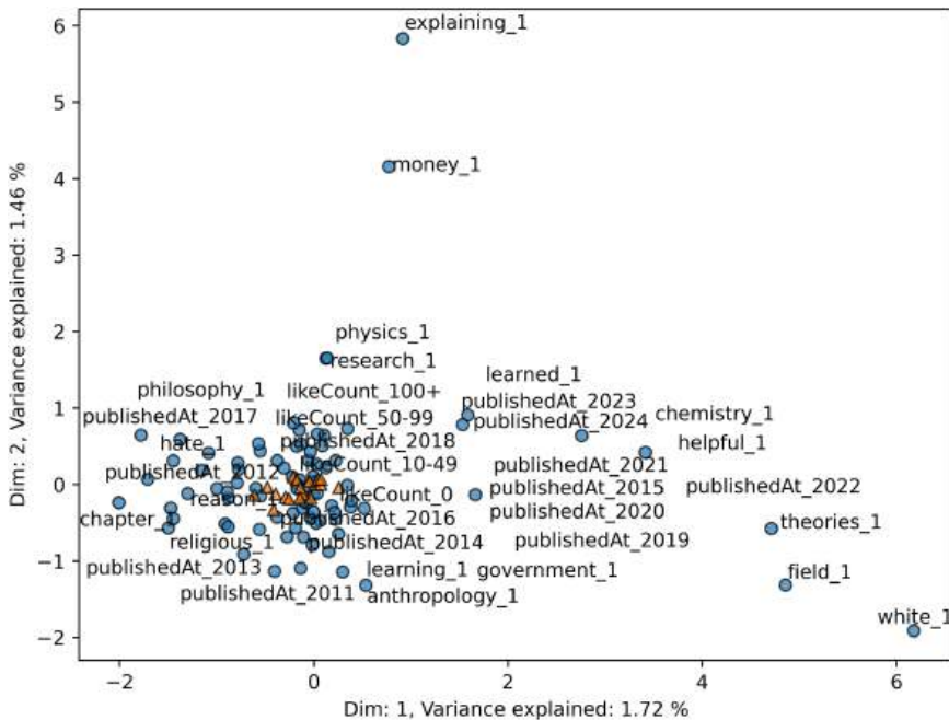
Figure 15.7 Biplot of the position of the active and passive variables on dimensions 1 and 2.
