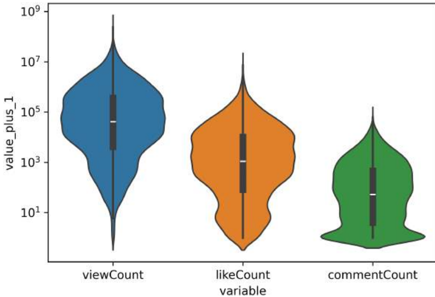
Figure 14.5 Violin plot of the number of views, likes, and comments per YouTube video.
