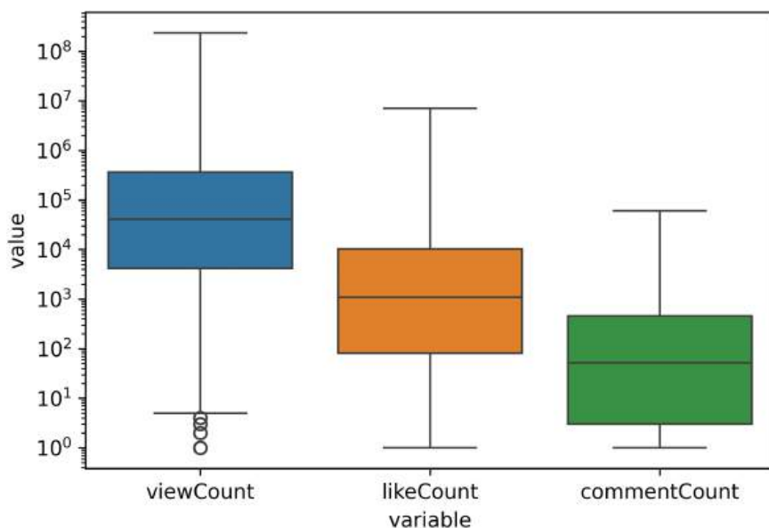
Figure 14.3 Boxplots of the three metric variables, with log-transformed y-scale.
