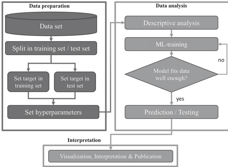
Figure 11.4 Idealized workflow with sequential, parallel, and recursive steps.
