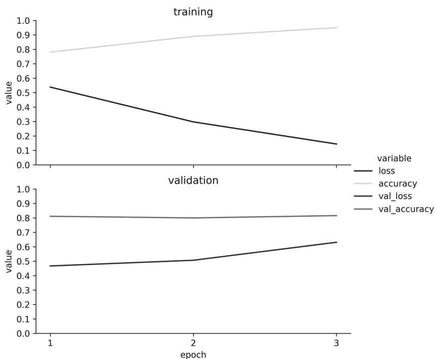
Figure 16.4 Visualization of the accuracy values and values of the loss function (categorical cross-entropy) in the training set and validation set.
