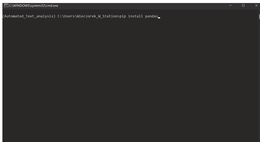
Figure 12.9 Command line with the pip command to install the package Pandas.
