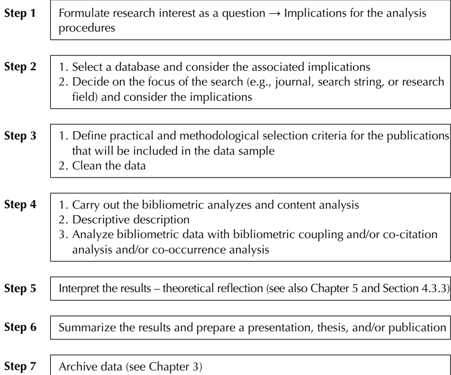
Figure 9.1 Flowchart of a bibliometric literature review.
