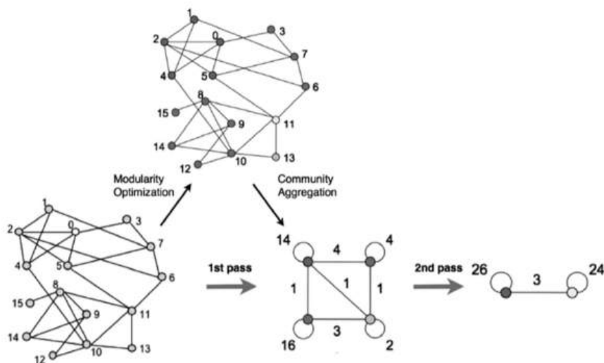
Figure 15.11 Visualization of the community detection algorithm.
