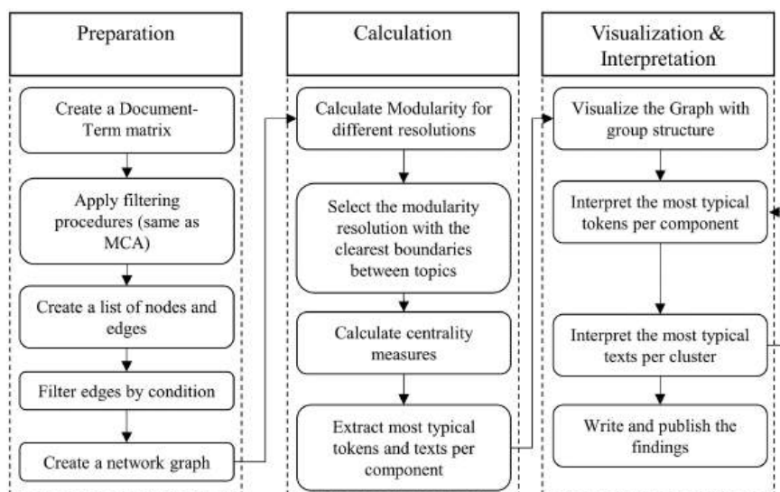
Figure 15.8 Workflow depicting the steps taken to conduct a semantic network analysis.
