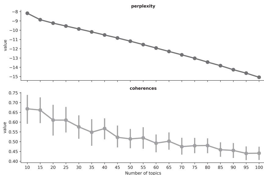
Figure 17.2 Perplexity und c_v coherence values per topic.
