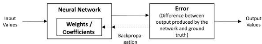
Figure 11.3 Schematic representation of the backpropagation algorithm (according to Werbos, 1990, S. 1552 slightly modified).
