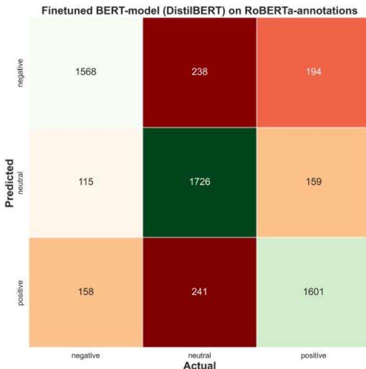
Figure 16.5 Confusion matrix of the predicted versus the actual sentiment classes of the test set.
