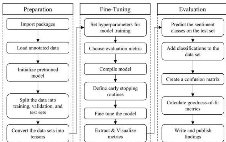
Figure 16.3 Workflow applied for fine-tuning the sentiment analysis and model evaluation.
