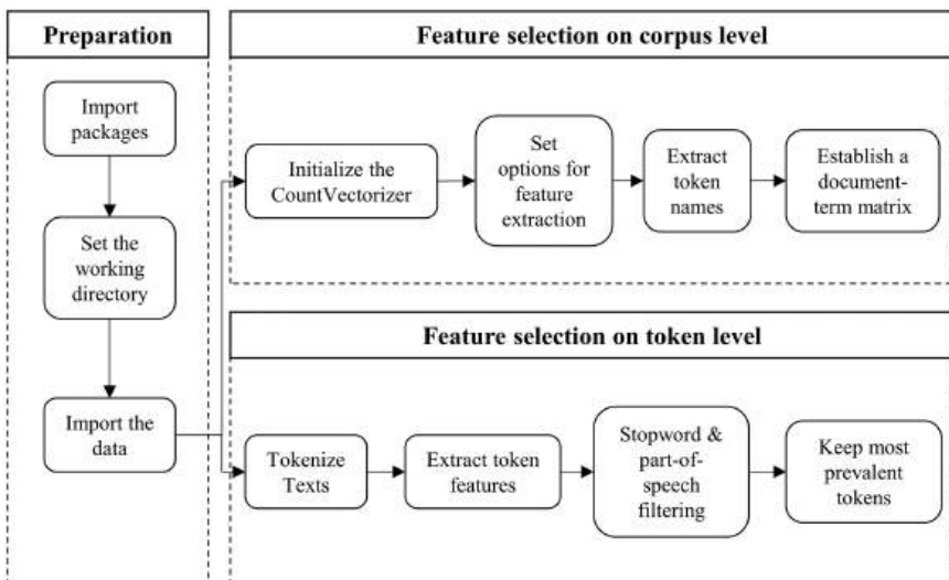
Figure 13.1 Workflow depicting the feature selection procedures on corpus level and on token level.
