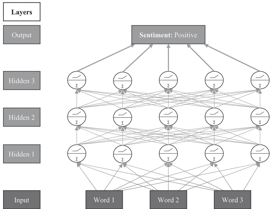
Figure 11.2 Depiction of a three-layer deep, fully connected artificial neural network (with ReLu activation function).
