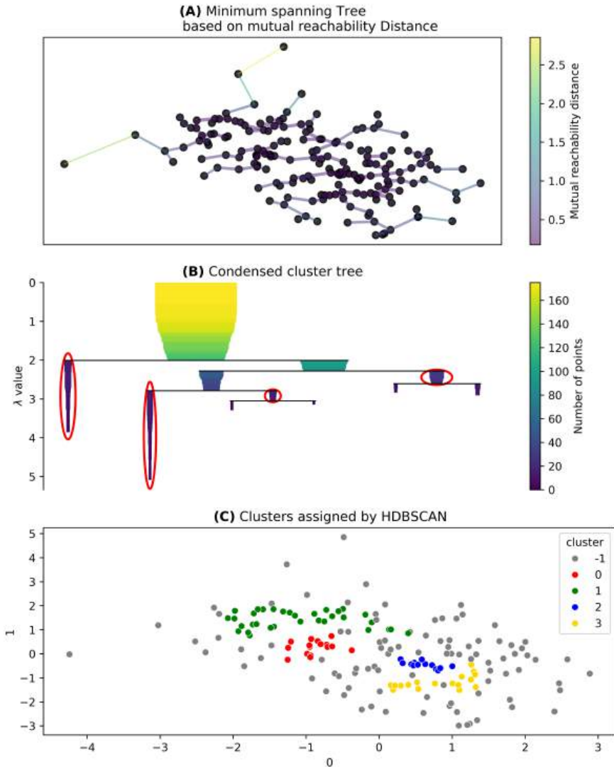
Figure 18.3 Depiction of the steps taken by HDBSCAN to cluster data.
