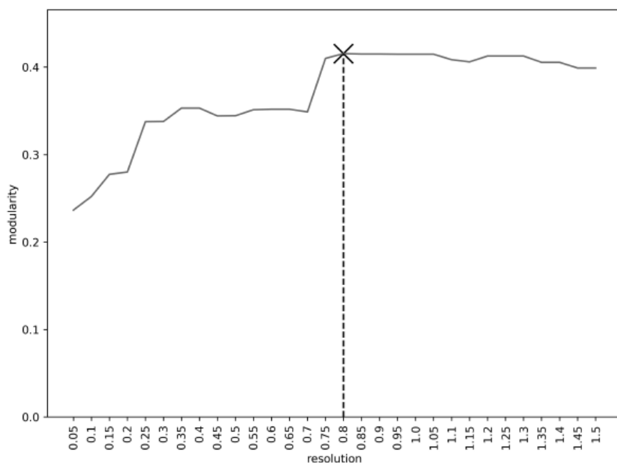
Figure 15.12 Line plot representing the extracted modularity value for each resolution parameter.
