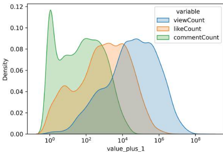
Figure 14.4 Kernel density plot of the number of views, likes, and comments per YouTube video.
