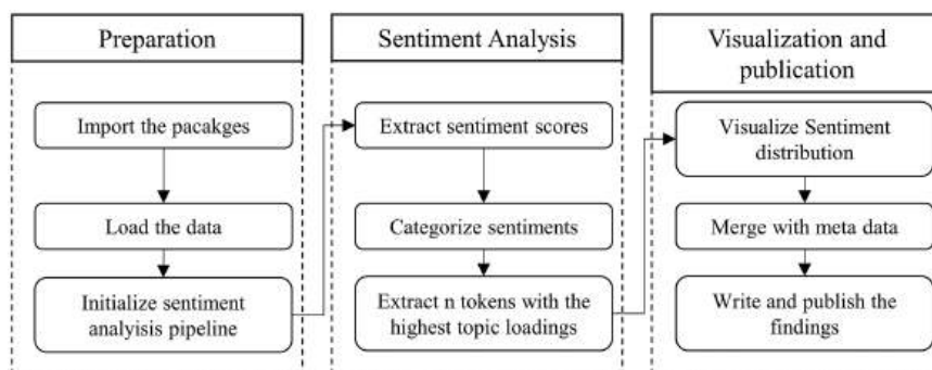
Figure 16.1 Workflow – lexical approach to sentiment analysis – VADER.
