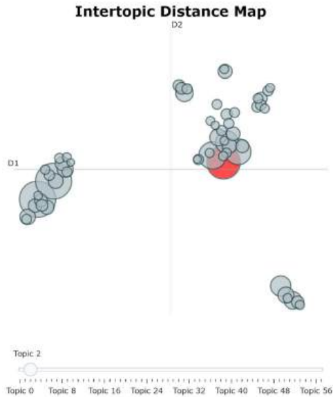
Figure 18.7 Intertopic distance map.
