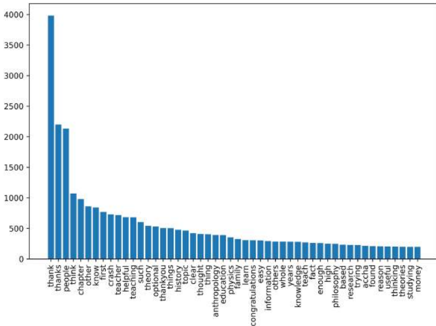
Figure 15.3 The 50 most frequent tokens in the document-term matrix of the YouTube comments regarding sociology videos.
