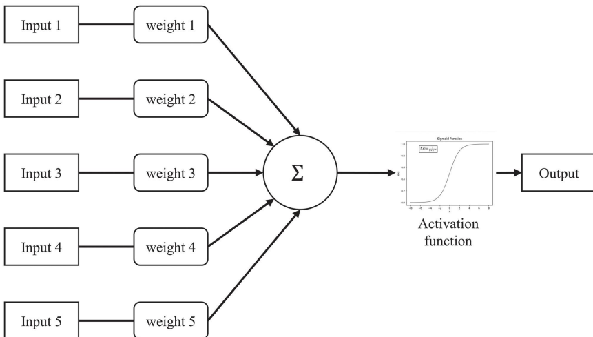
Figure 11.1 Stylized depiction of a perceptron with a sigmoid activation function.
