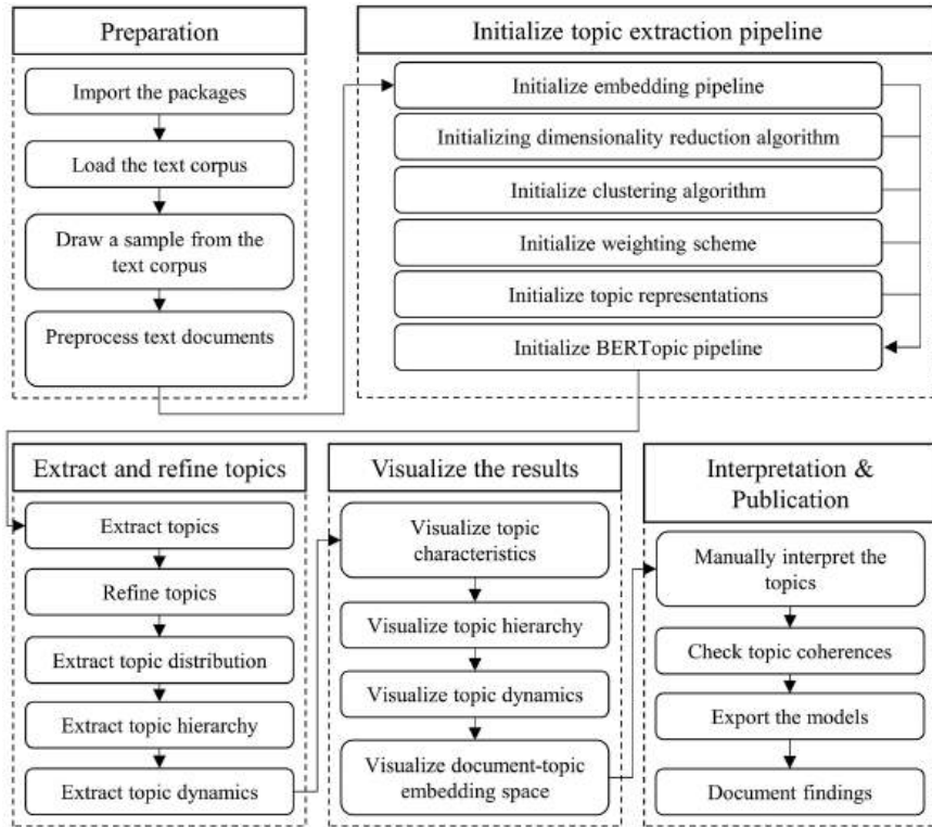
Figure 18.1 Workflow depicting the steps taken for topic modeling with BERTopic.
