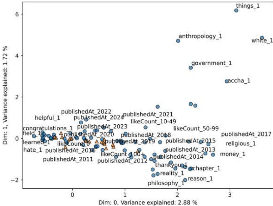
Figure 15.5 Biplot of the first two dimensions extracted by the MCA from the document-term matrix.
