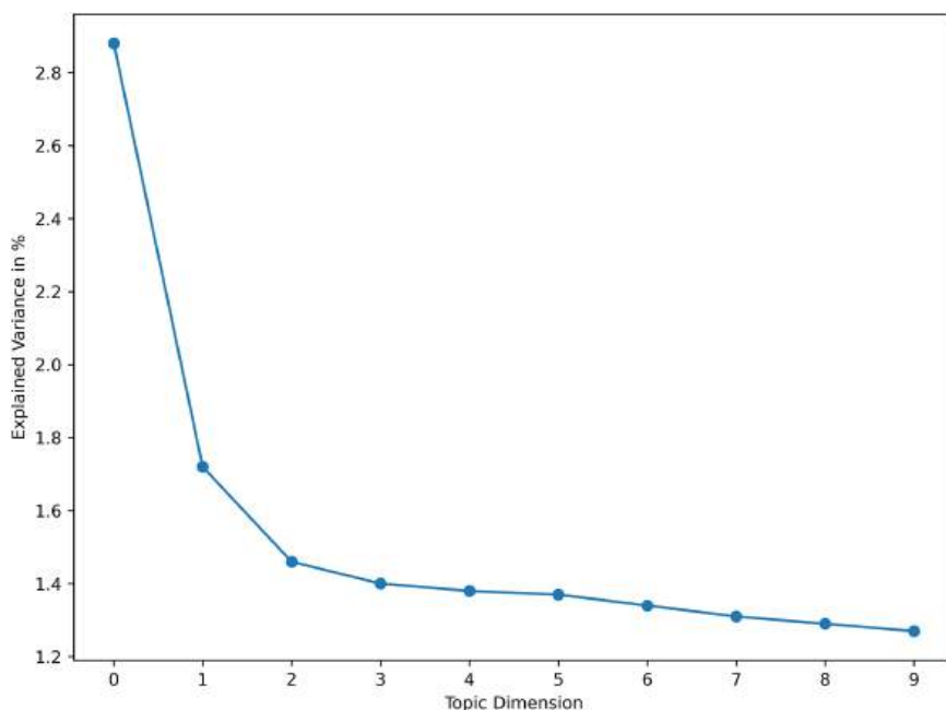
Figure 15.4 Scree plot of the variables explained by topic dimension extracted by the MCA.
