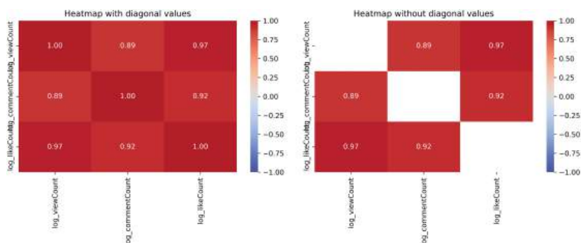
Figure 14.9 Heatmap of the pairwise correlations between the number of views, comments, and likes of the YouTube videos under observations with and without diagonal.
